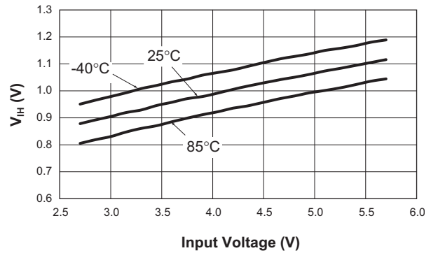
V_{IH} vs. Input Voltage
