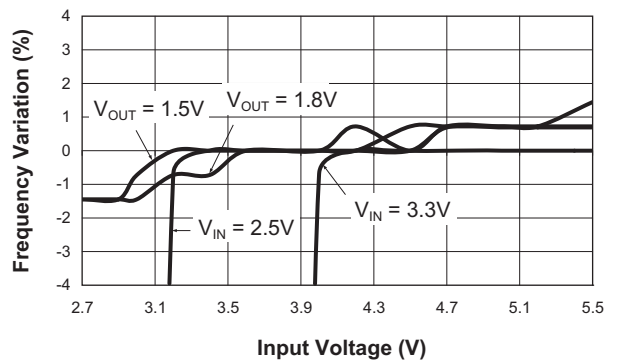
Switching Frequency vs. Input Voltage ( I_{OUT} = 600mA ; 25°C)
